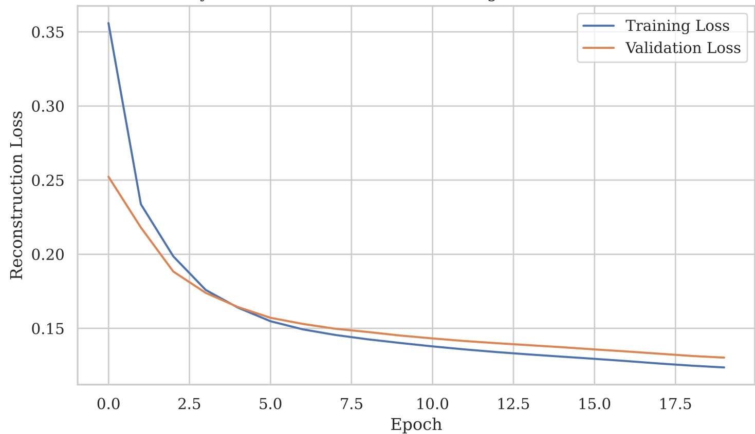
Fully Connected Autoencoder: Training and Validation Loss
